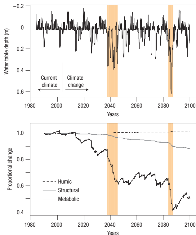
Figure 4 Transient change in the water table at the BOREAS Fen site, 2004–2099. a , Change in water table. b , Proportional changes in SOC. Before 2004, the model is in equilibrium under the 1994–2005 climate. Then, temperature and precipitation anomalies projected by HadCM3 with Special Report on Emissions Scenarios A2 are used to force the model in and after year 2004. Shaded areas denote extremely dry periods of 2038–2045 and 2084–2087.
